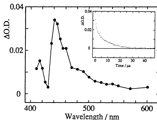
Fig. 4. Transient absorption spectrum in benzene with a decay curve.
